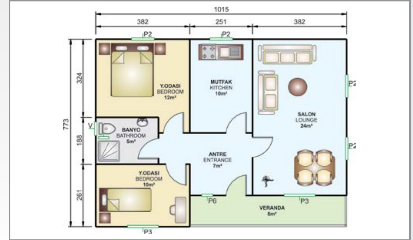
PREFABRİK KONUT PLANLARI (78m 2 ) Prefabricated House Plan (78m 2 )
