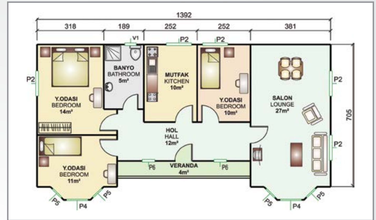
PREFABRİK KONUT PLANLARI (98m 2 ) Prefabricated House Plan (98m 2 )
